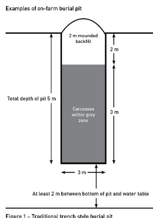
Figure 1 – Traditional trench style burial pit
