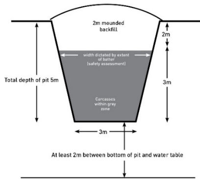
Figure 2 – Battered burial pit
